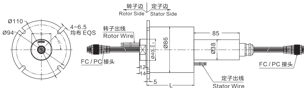
FO608 series 6 channels Fiber-Electric slip ring model selection table
